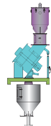
二次侧材料混合贮存料斗 Secondary Mixed material Storage tank
