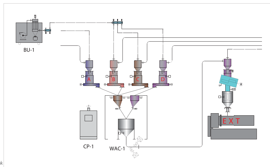
二次侧材料混合贮存料斗 Secondary Mixed material Storage tank
